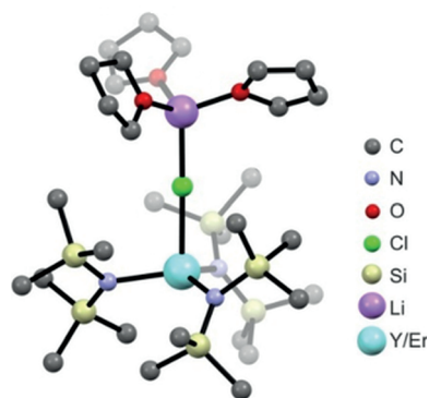
Figure 4. Molecular structure of [\text{Er}_{0.1}\text{Y}_{0.9}\{(\text{Me}_3\text{Si})_2\text{N}\}_3(\mu\text{-Cl})\{\text{Li}(\text{THF})_3\}]\cdot \text{pentane} ( 1' ). Hydrogen atoms and pentane molecules were omitted for the sake of clarity.
